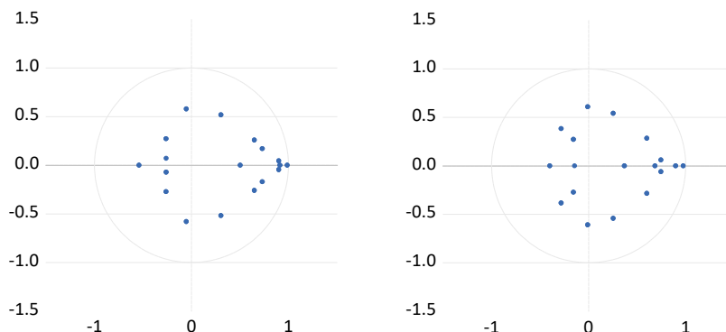
Inverse Roots of AR Characteristic Polynomial
